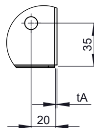
DETAILB (1 : 3)
