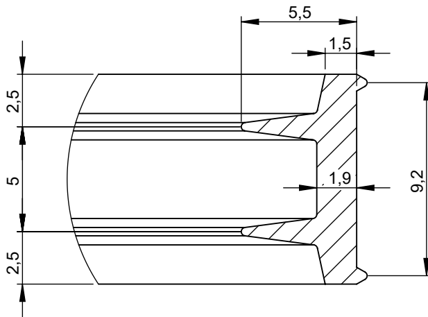
DETAILB (4 : 1)
